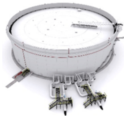
Vertical steel tank with floating roof (PBCПк)
