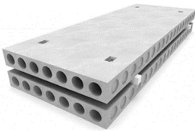
PB and PK hollow-core slabs of up to 9 m length and 1.2 m and 1.5 m width
